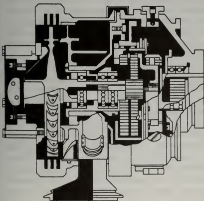
FIGURE 5-17. Cutaway of an air turbine starter.
